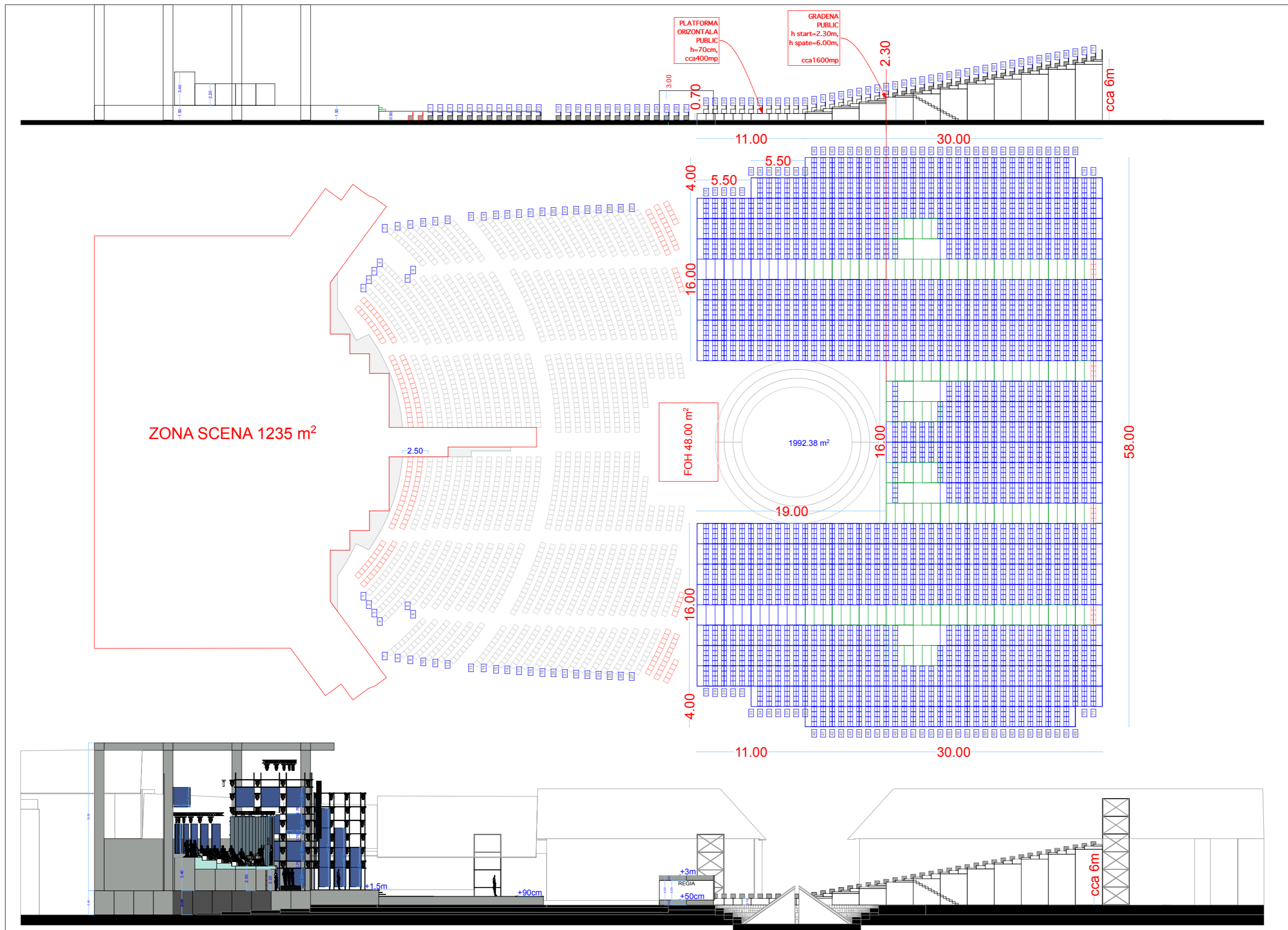
PS 1 CERBUL DE AUR - 2018 PLANSA AMENAJARE GRADENE PUBLIC
